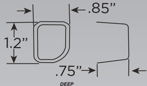
Multi-Dose Blister Dimensions
